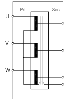
• Circuit Diagram
