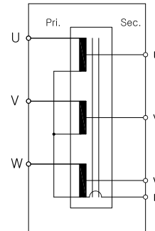
• Circuit Diagram
