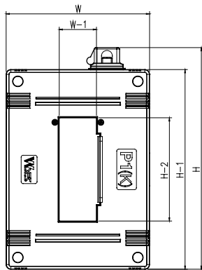
WV Type (Vertical Type)
