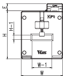
CS "A" TYPE
