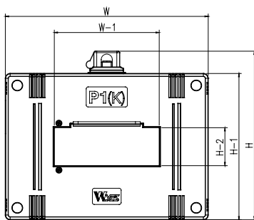
WH Type (Horizontal Type)
