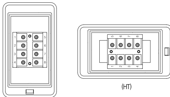
Terminal type
