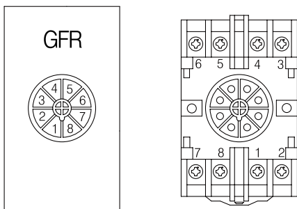
Socket type
