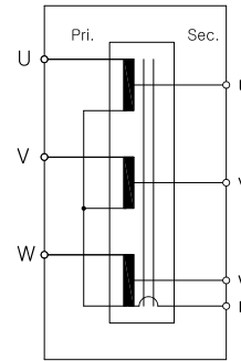
• Circuit Diagram
